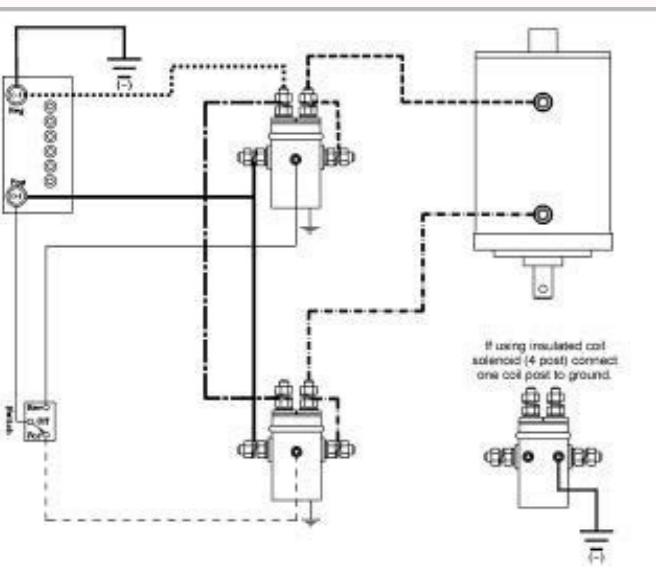
(Late Wiring Design) Permanent magnet bi-directional motor
